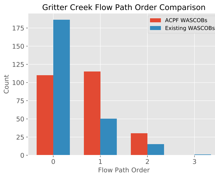
Figure 3.13: Gritter Creek WASCObS Flow Path Order Comparison.
