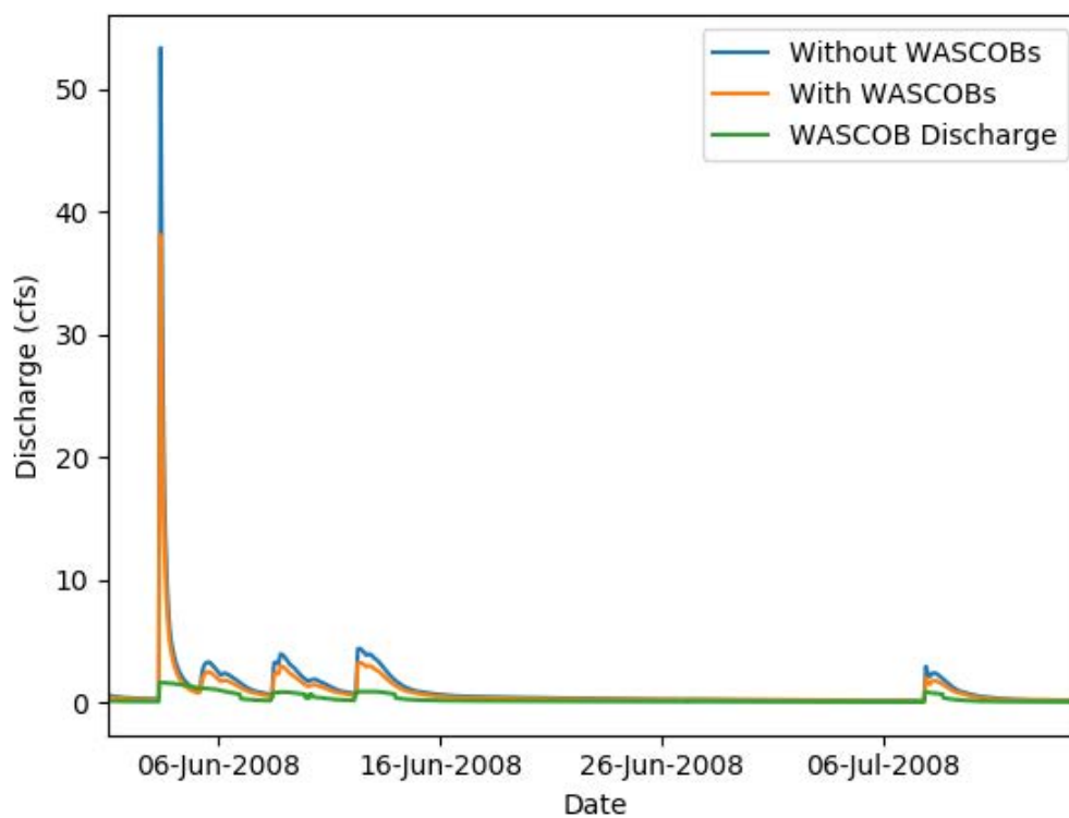
Figure 6.6: Single Subbasin Event Analysis. Hourly discharges for the 2008 flood with the original model (blue), with WASCObS included (orange), and just the WASCOb outlet (green).
