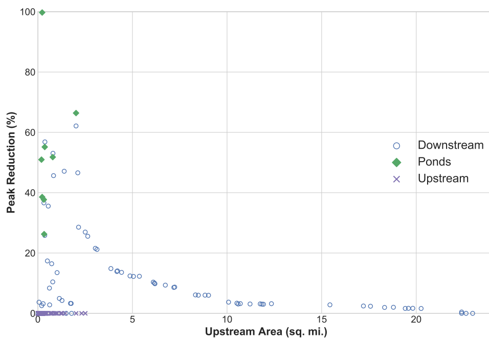
Figure 5.12: Gritter Creek Peak Reduction with ACPF NRW. Average peak reduction for each subbasin in Gritter Creek. The points are labeled by whether they are upstream of ponds, at the site of a pond, or downstream of ponds.
