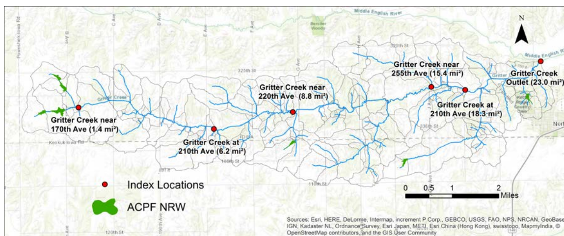
Figure 5.6: Gritter Creek Index Locations. Location of the six selected index points for Gritter Creek, also showing the locations of NRW.
